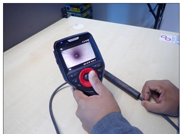
Aid visual on internal defected tube using borescope equipment.
